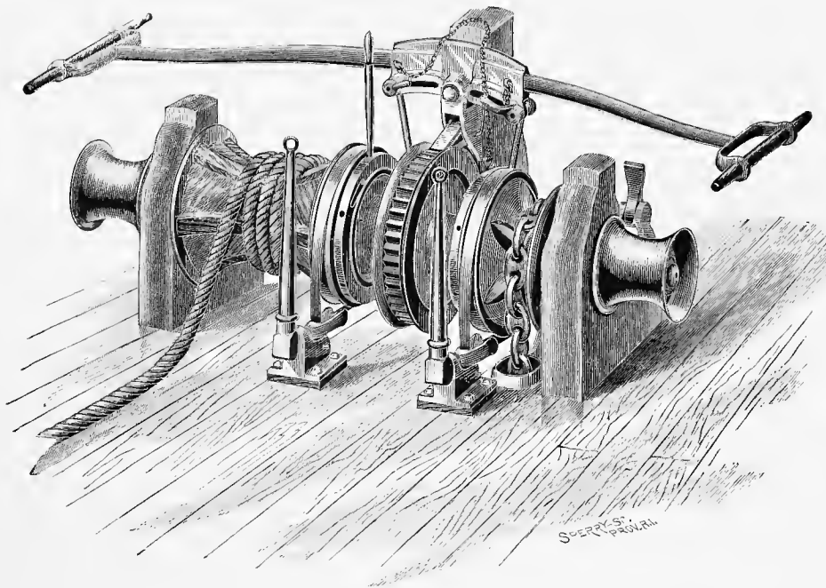
PROVIDENCE FISHERMAN'S WINDLASS.—Built by the American Ship Windlass Co.
